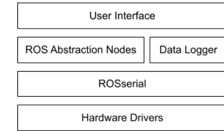
Fig. 11. Software Stack
