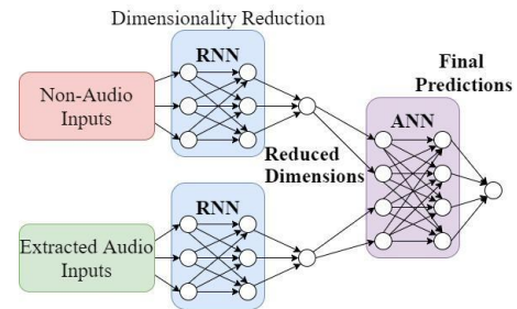
Fig. 16. Hive Architecture
