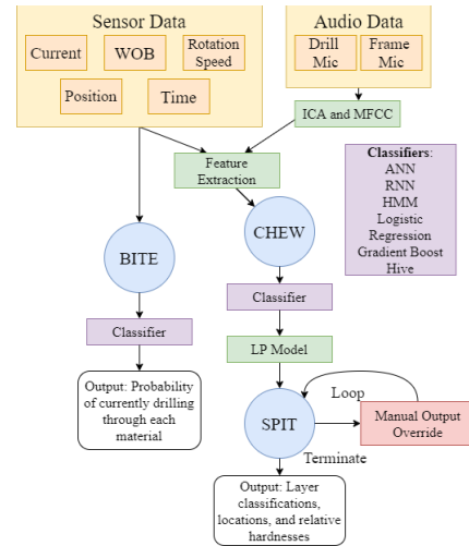
Fig. 15. Digital Core Flow and Hierarchy
